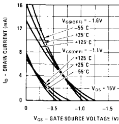
Transfer Characteristics
