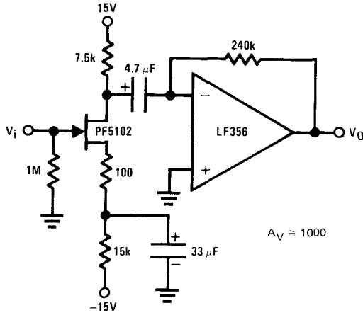
a. Single-Ended
