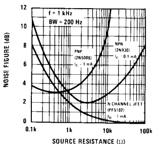
FIGURE 1. Bipolar and JFET Transistor Noise Comparison
