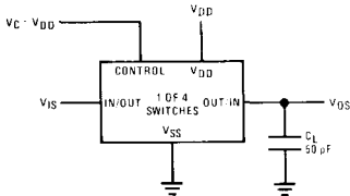
FIGURE 1. t_{pHL} , t_{pLH} Propagation Delay Time Signal Input to Signal Output
