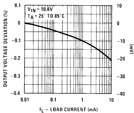
FIGURE 3. Load Regulation
