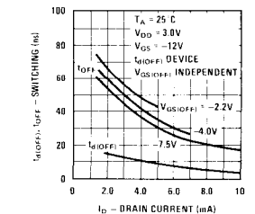
Turn-Off Switching
