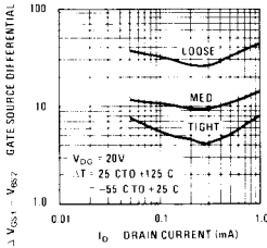
Differential Drift
