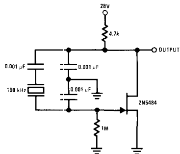
Stable Low Frequency Crystal Oscillator
