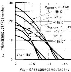
Transfer Characteristics
