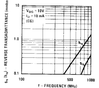
Reverse Transmittance
