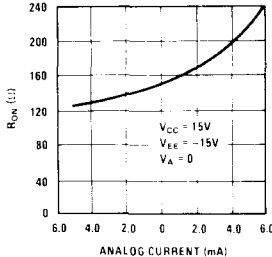
"ON" Resistance
