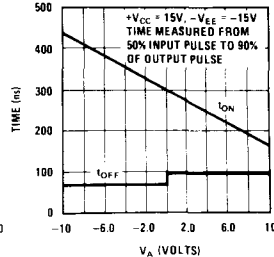
Break-Before-Make Action
