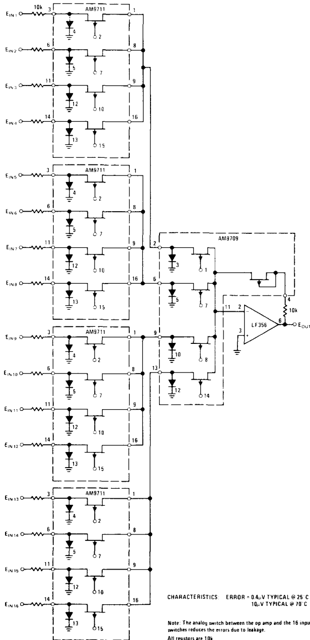
16-Channel Multiplexer
