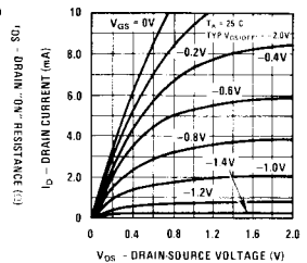
Common Drain-Source Characteristics
