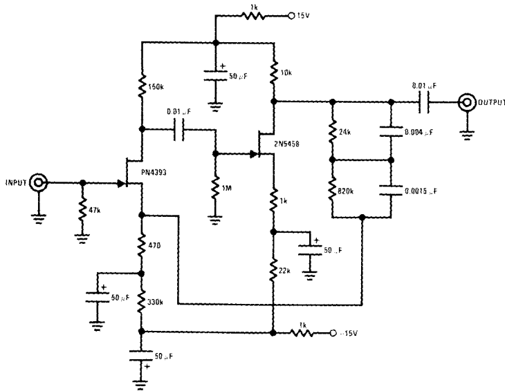
Magnetic Pickup Phono Preampifier
