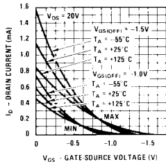
Transfer Characteristics
