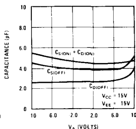
Switch Capacitances
