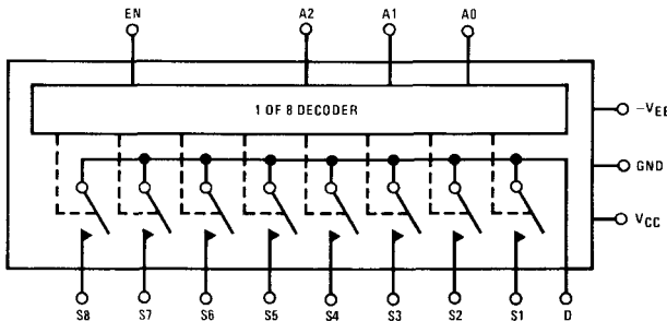
LF11508/LF12508/LF13508
