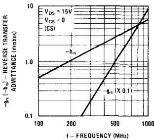
Reverse Transmittance
