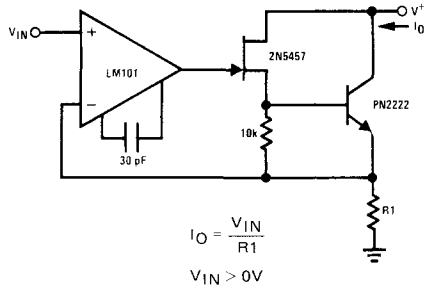
Precision Current Sink
