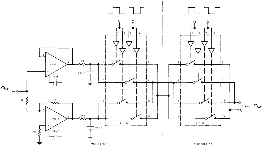
DSB Modulator-Demodulator
