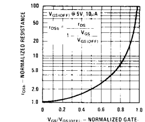
Normalized Drain Resistance vs Bias Voltage
