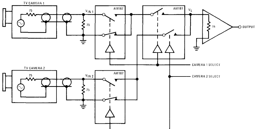
Video Switch with Very High "OFF" Isolation (f = dc to 10 MHz)
