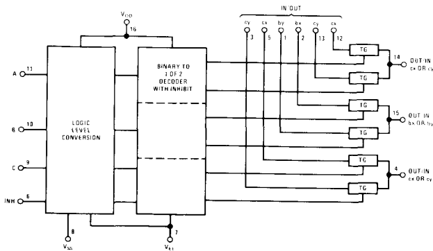
CD4053M/CD4053C
