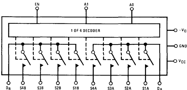
LF11509/LF12509/LF13509
