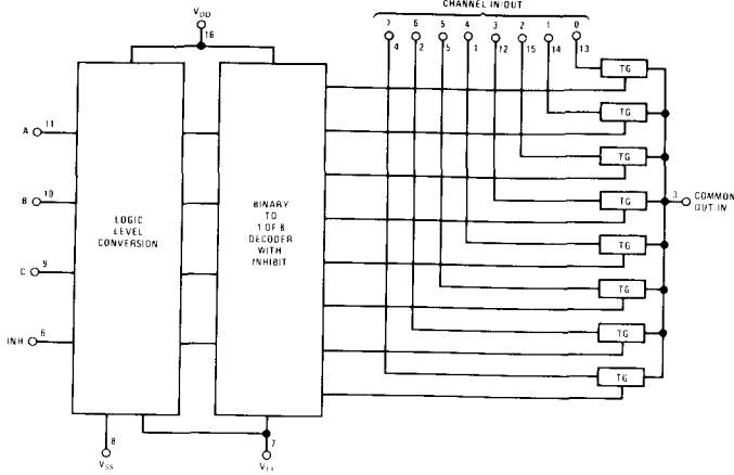
CD4051M/CD4051C
