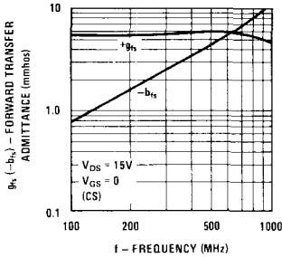
Forward Transmittance
