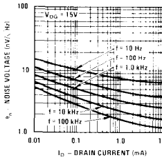
Noise Voltage vs Current
