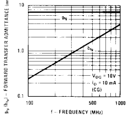
Forward Transadmittance
