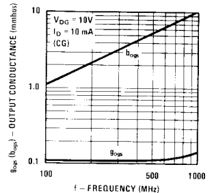
Output Admittance
