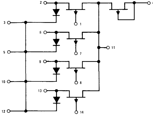
14-Pin DIP
