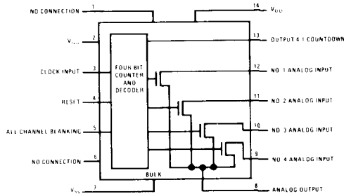
Flat Package
