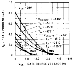
Transfer Characteristics
