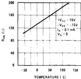
"ON" Resistance
