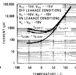
Switch Leakage Currents
