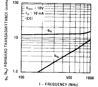
Forward Transmittance
