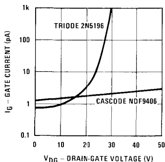
FIGURE 2. Typical Gate Current vs Drain-Gate Voltage @ I_D = 200 \mu A
