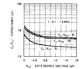
Capacitance vs Voltage
