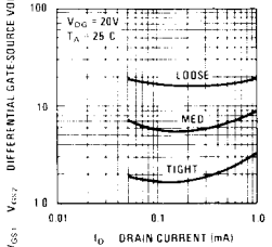
Differential Offset
