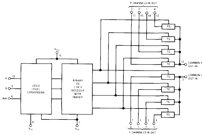
CD4052M/CD4052C
